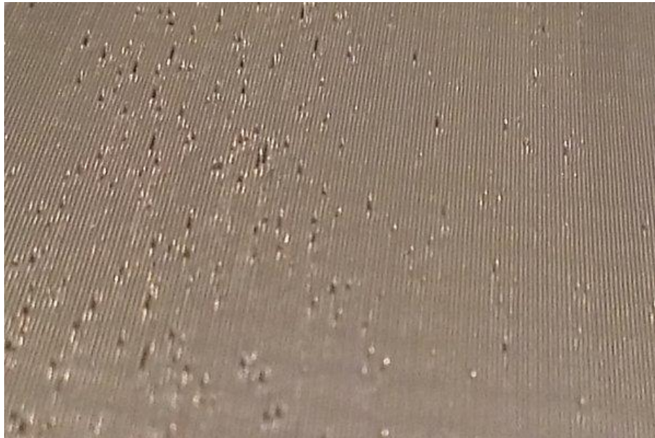
Voids in 3D Printed parts. Source: idig3dprinting.com
