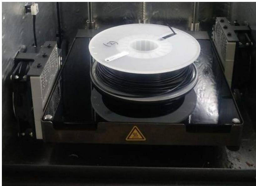
A filament being dried inside a heated 3D printer chamber.
